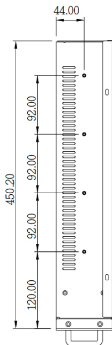
Left-side View
