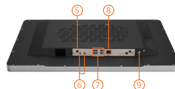
▲ SDM-L slot
